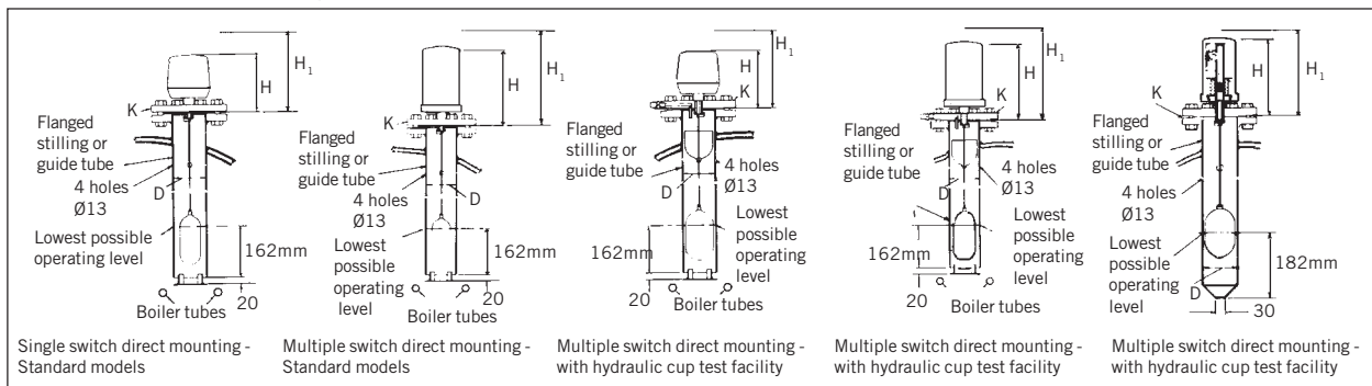
Fig. 7 Hydraulic cup test facility model
