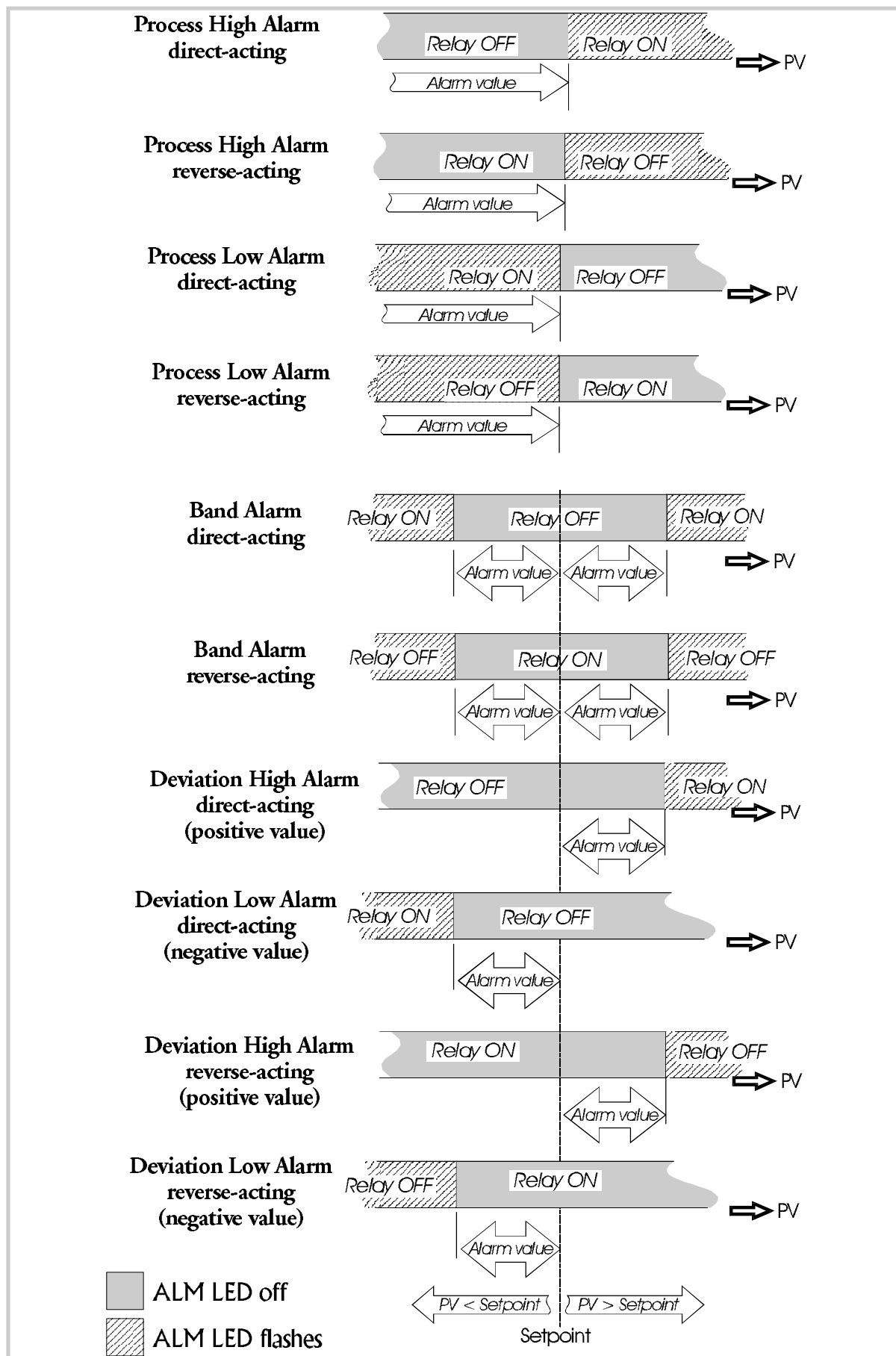
Figure 2-2 Alarm Operation
